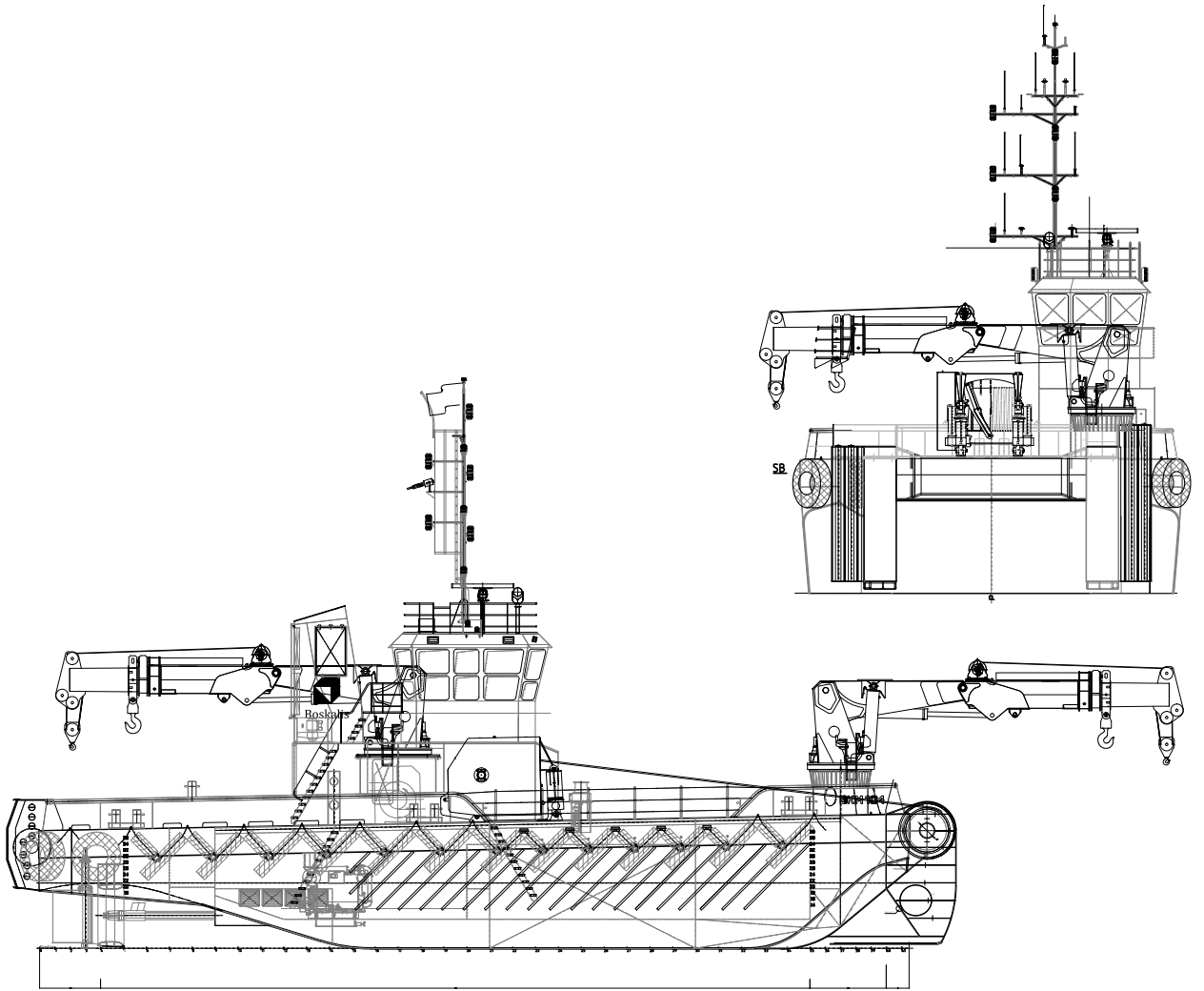
SIDE VIEW
