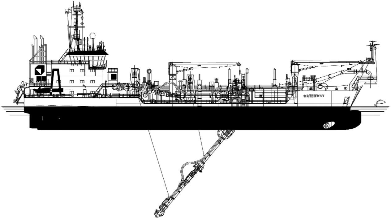
SIDE VIEW
