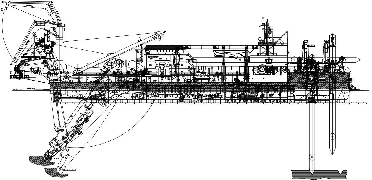
SIDE VIEW
