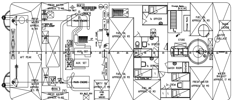
TOP VIEW DECK LEVEL
