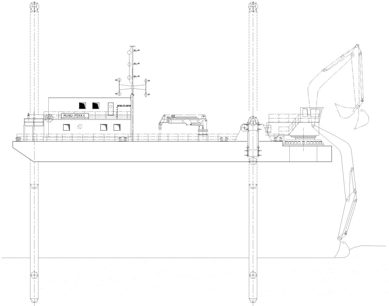
SIDE VIEW
