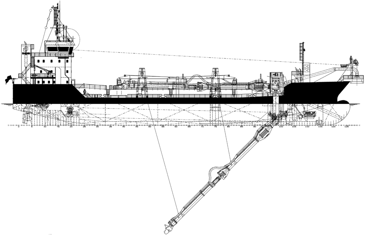
SIDE VIEW
